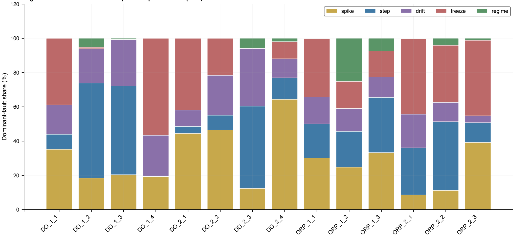
Figure 6. Dominant fault decomposition per channel (v1.1)
